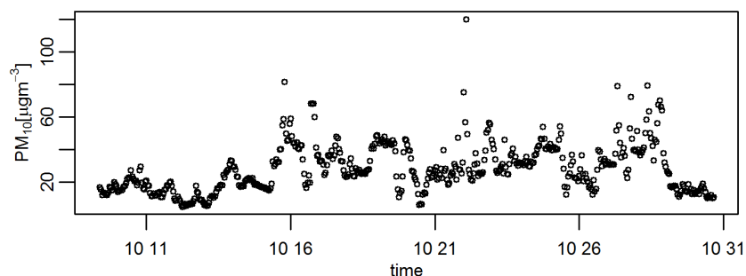
1: Concentrations of \text{PM}_{10} aerosols
