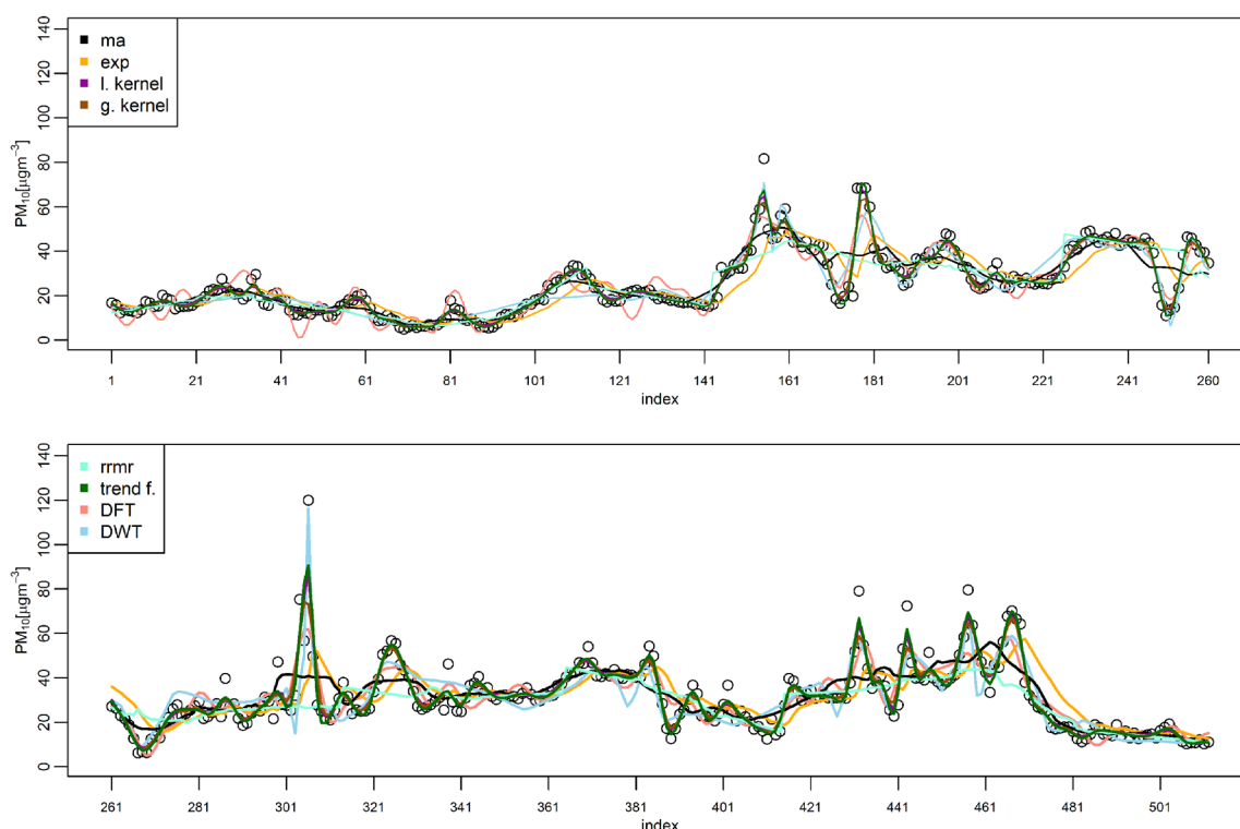
2: Concentrations of PM_{10} aerosols together with the smoothing lines obtained using: moving average (ma), exponential smoothing (exp), local kernel regression (l. kernel), global kernel regression (g. kernel), robust repeated median regression (rrmr), trend filtering (trend f.), discrete Fourier transform (DFT) and discrete wavelet transform (DWT)
