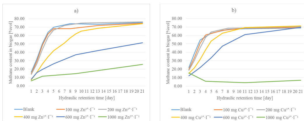
2: Methane content in biogas during experiment No. 1 (a) and No. 2 (b)
