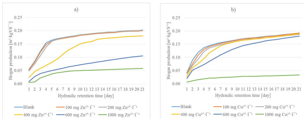
1: Cumulative biogas production during experiment No. 1 (a) and No. 2 (b)
