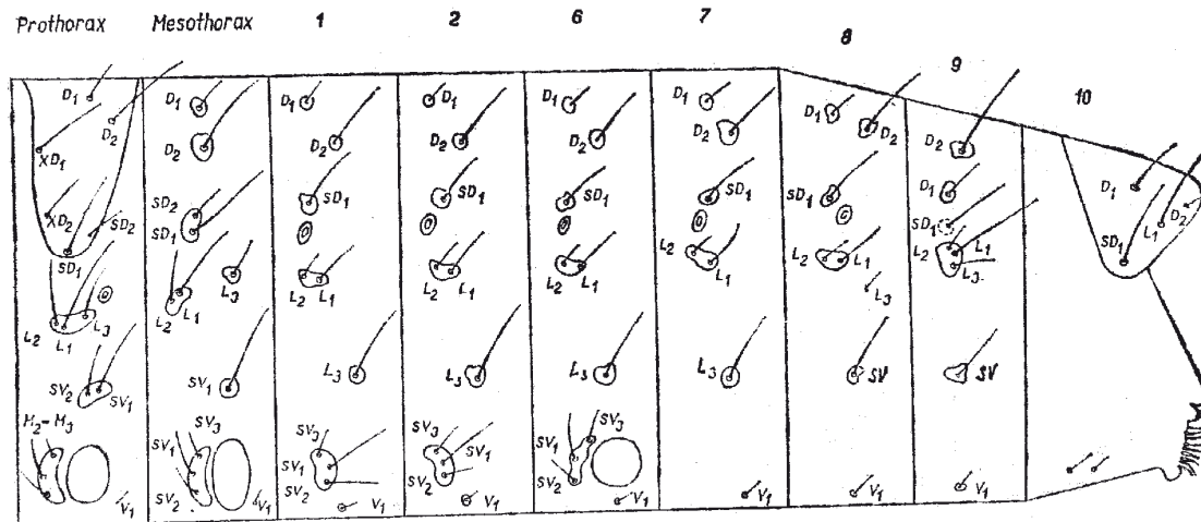
6: General scheme („map“) of caterpillar chaetotaxy in gnorimoschemine moths showing all groups of setae. In specialized taxa (leaf-miners, gall-producers) a tendency towards the chaetotaxy reduction is observed.
