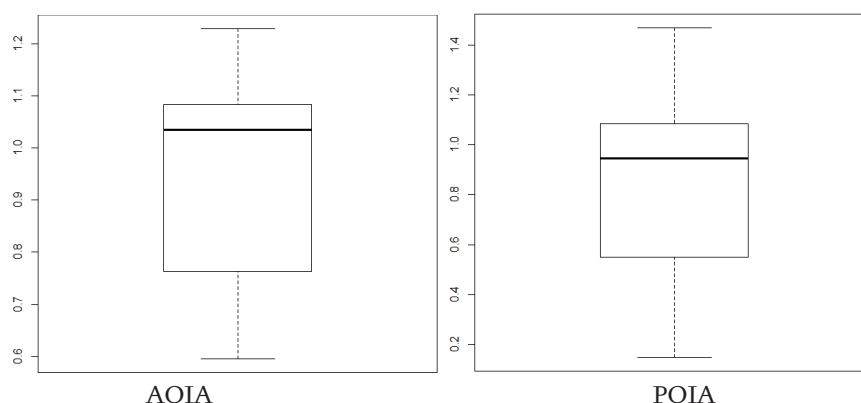
4: Boxplot of super-efficiency scores under the asset-oriented intermediation approach (AOIA) and profit-oriented intermediation approach (POIA) without outliers
