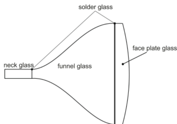
1: Main glass components of a typical cathode ray tube
